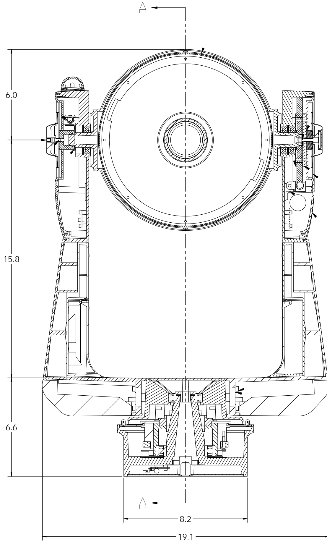
SECTION B-B SCALE 0.500
